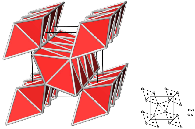
\beta -BeO
