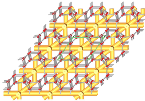
Phillipsit (PHI) 5
