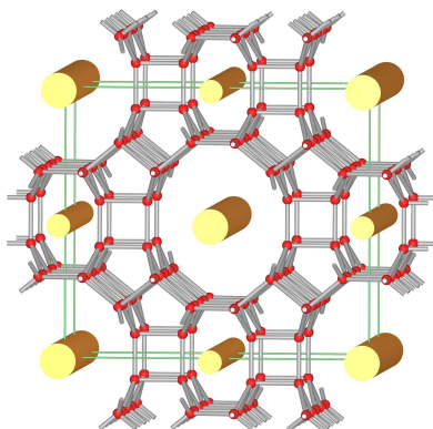
Mordenit (MOR) 10
