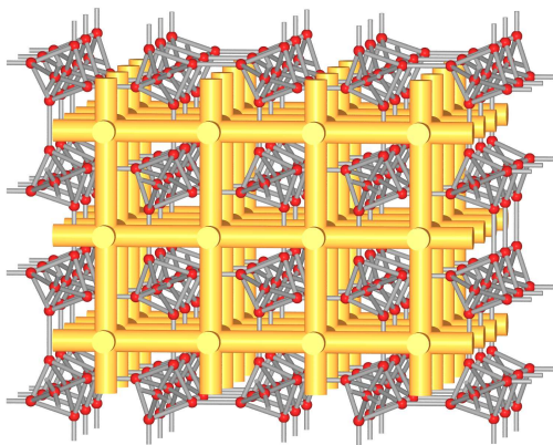
Thomsonit (THO) 2
