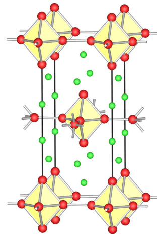
\text{Cs}_2\text{In}_3
